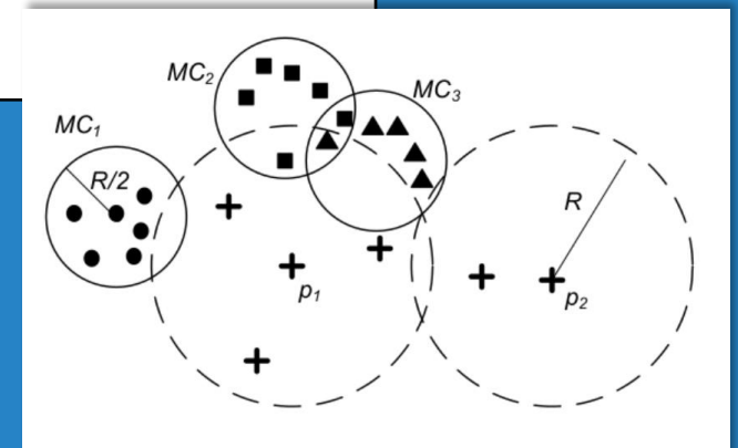
Fig. 4. MCOD - Micro-clusters.
